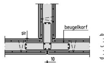
Detail H3 - principedetail T-hoek
