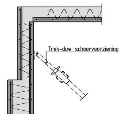
Detail V3 - principedetail wandverjonging
